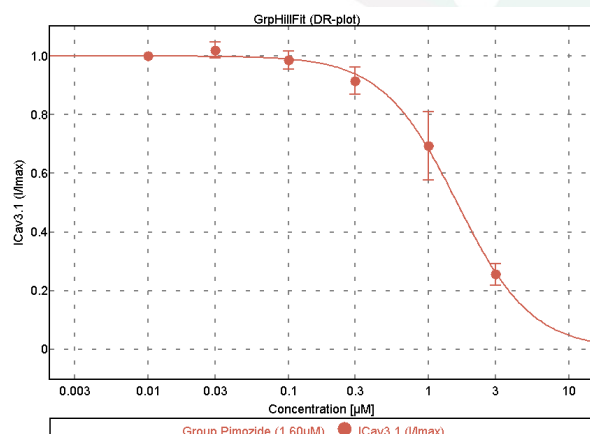
Figure 2: Concentration-dependent effects of Pimozide on I Ca currents (pA) obtained from HEK-293 cells stably transfected with human Ca v 3.1 channels. Calculated IC 50 value was approximately 1.60 µM (n=3).
