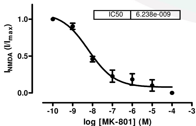
Figure 2: Concentration dependent effect of antagonist MK-801. Calculated IC 50 value was approximately 6.2 nM (n=2).
