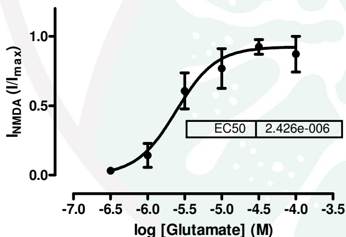
Figure 1: Concentration dependent effect of agonist Glutamate (co-applied with 10 \mu M Glycine) Calculated EC 50 value was approximately 2.4 \mu M (n=3).
