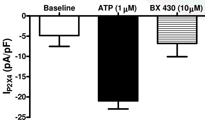
Figure 2: Inhibitory effect of antagonist BX 430 (10 μM) on the ATP-induced activation obtained from HEK-293 cells stably expressing P2X4 channels .
