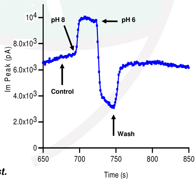
Figure 2: Time-course of the effect of pH 8 (activator) and pH 6 (inhibitor) on TASK-1 expressing cells.
