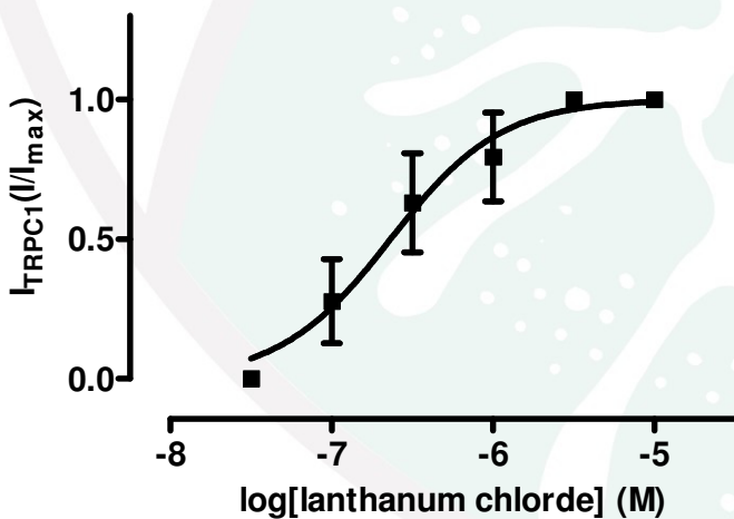
Figure 1: Plotted graph of normalised concentration-response activation curve of lanthanum chloride against the hTRPC1 channel. Calculated EC 50 value was approximately 0.2μM (n=5).
