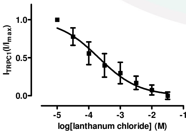
Figure 2: Plotted graph of normalised concentration-response inhibition curve of lanthanum chloride against the hTRPC1 channel. Calculated IC 50 value was approximately 207μM (n=3).
