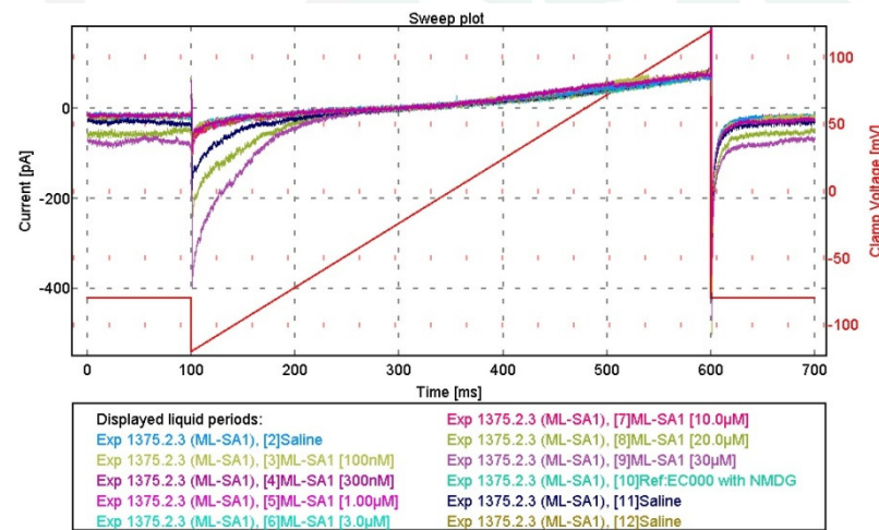
Figure 1: Representative example of superimposed voltage and current traces showing inward and outward TRPML3 current in the presence of agonist ML-SA1.
