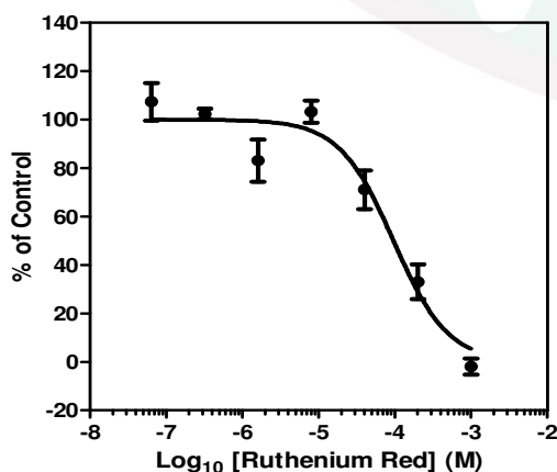
Figure 2: Dose response curve of antagonist ruthenium red against guinea pig TRPA1 using calcium sensitive dye assay. IC_{50} value 95.8 \mu\text{M} .
