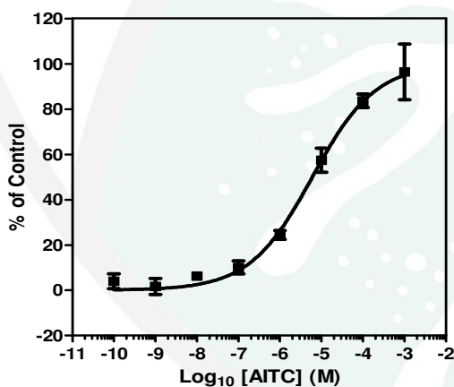
Figure 1: Dose response curve of agonist AITC against guinea pig TRPA1 using calcium sensitive dye assay. EC_{50} value 6.03 \mu\text{M} .
